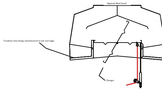
End View Cable operation
