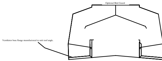
End View Permanently venting.
